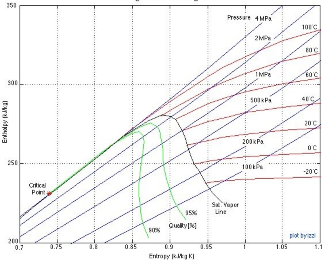
h-s diagram for R134a refrigerant
